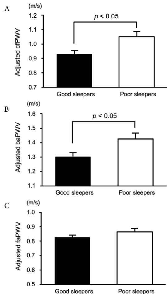
Figure 1 Carotid-femoral PWV (A), brachial-ankle PWV (B), and femoral-ankle PWV (C) values for good sleepers and poor sleepers. Differences in PWV between good sleepers and poor sleepers were assessed by a covariance analysis model that included age, blood pressure, and physical activity as covariates. Data are expressed as mean ± SE.
