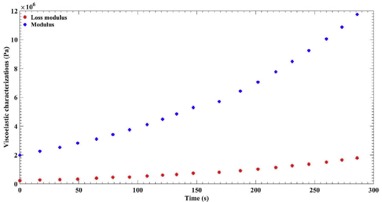
Figure 5 Alterations of the loss modulus and modulus of the SSV versus the time in tension.
