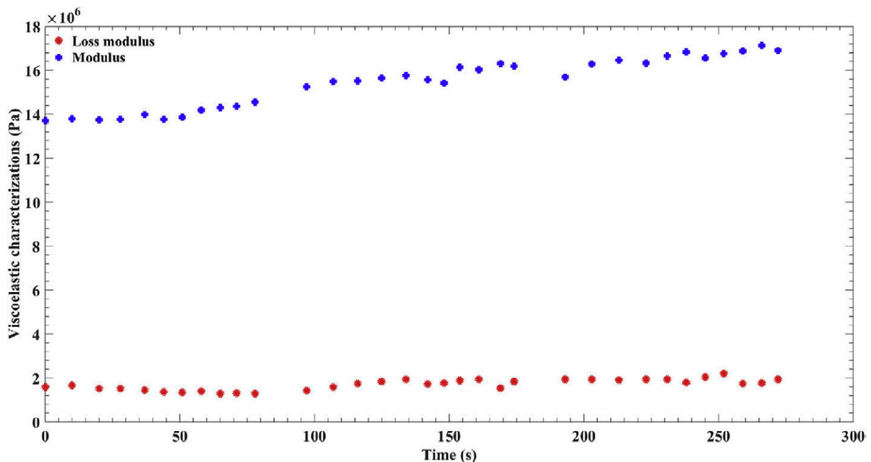
Figure 4 Alterations of the loss modulus and modulus of the SSV versus the time in compression.
