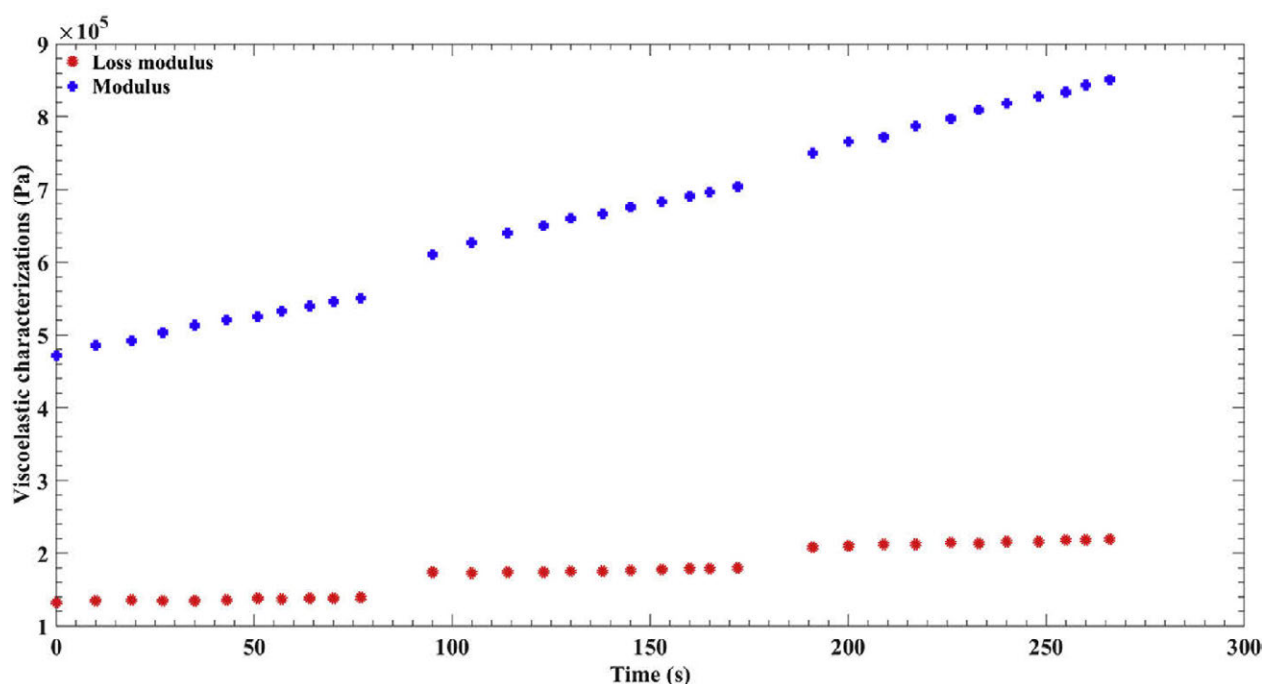
Figure 2 Alterations of the loss modulus and modulus of the ITA versus the time in compression.
