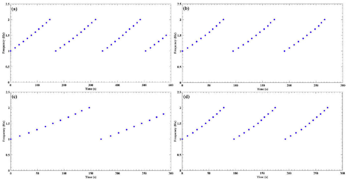
Figure 1 Alterations of the loading frequency versus the time in all tests, including the (a) ITA tension, (b) ITA compression, (c) SSV tension, and (d) SSV compression.
