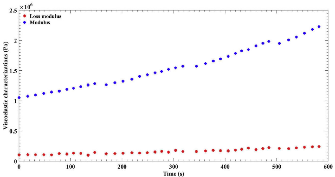
Figure 3 Alterations of the loss modulus and modulus of the ITA versus the time in tension.
