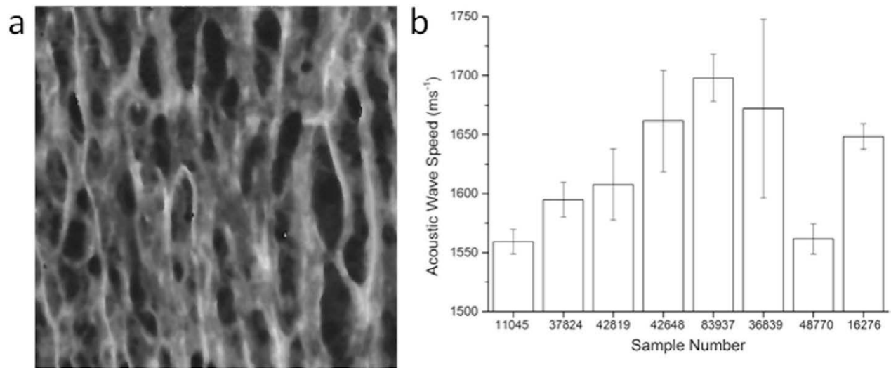
Figure 2 a) 200 \times 200 \mu\text{m} SAM image of the medial layer for Sample 37824; b) Mean values for acoustic wave speed as determined by SAM for the different samples tested. Error bars represent standard deviation.
